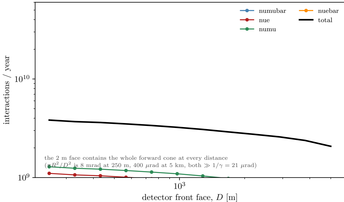
SM neutrino interactions vs detector location (both beams, HPGAr + 3 W slabs, r = 2 m)
