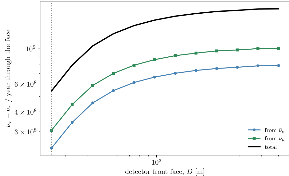
Secondary \nu_\tau vs detector location
