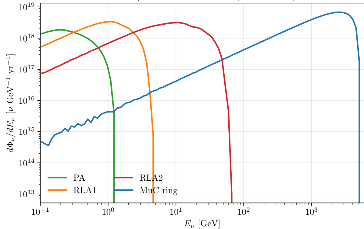
Total \bar{\nu}_\mu production spectrum (all directions)
