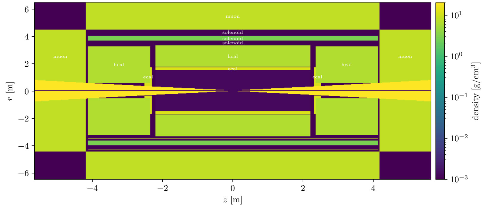
Muon-collider detector: material distribution
