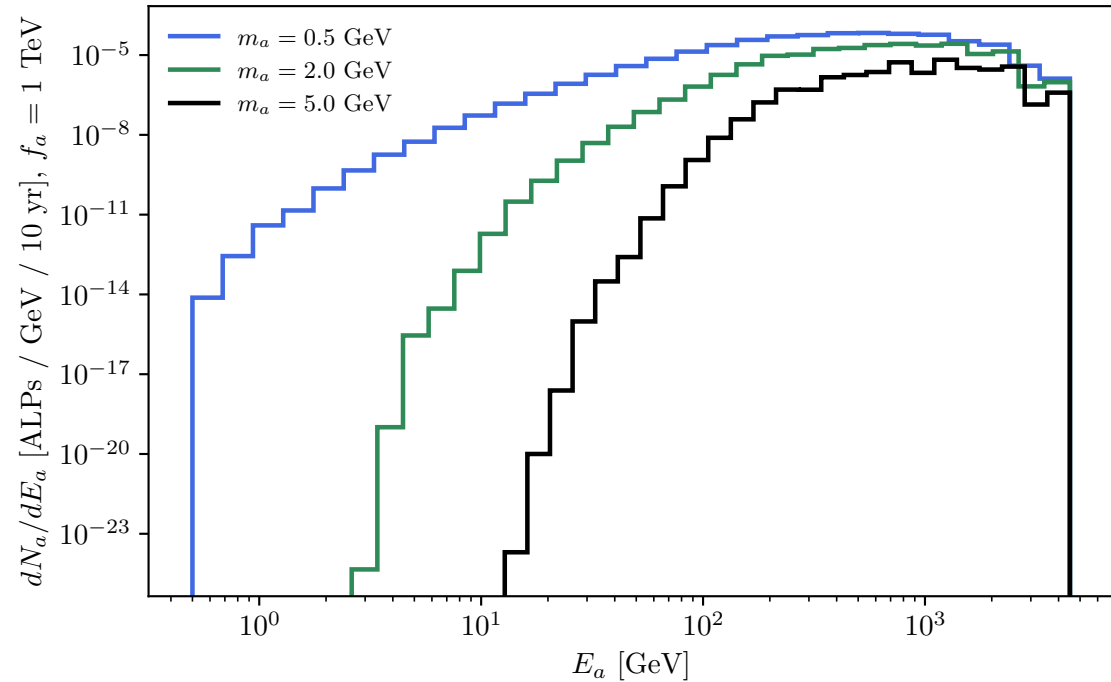
produced-ALP spectrum (flux-folded)
