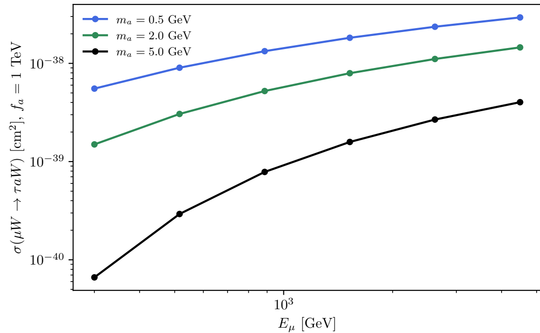
production cross section (exact 2→3, coherent Helm)
