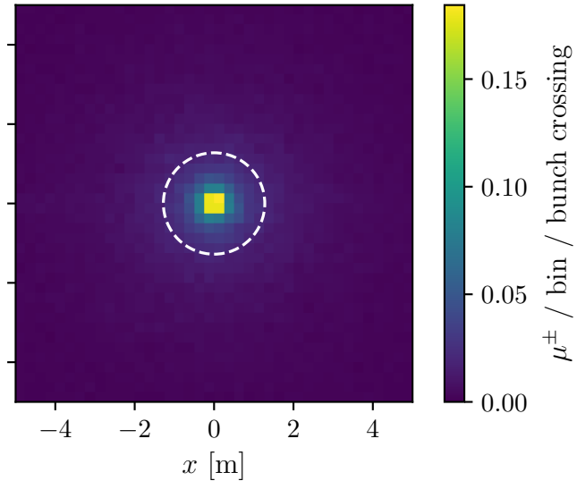
\mu^- beam, beam dyn. off
