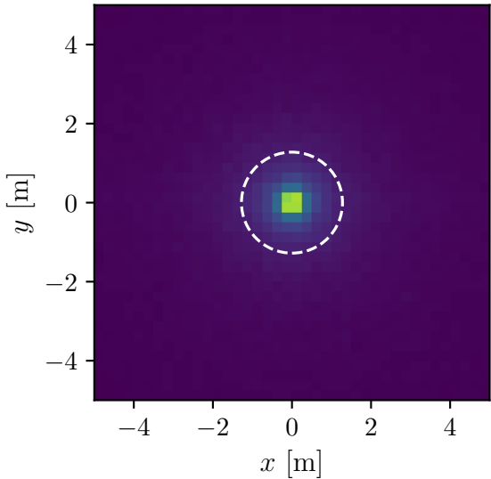
\mu^+ beam, beam dyn. off
