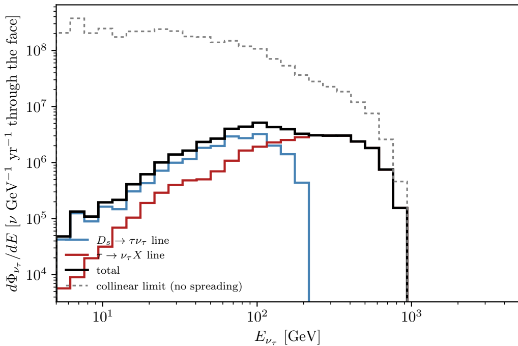
Secondary \nu_\tau + \bar{\nu}_\tau flux at L = 5 km
