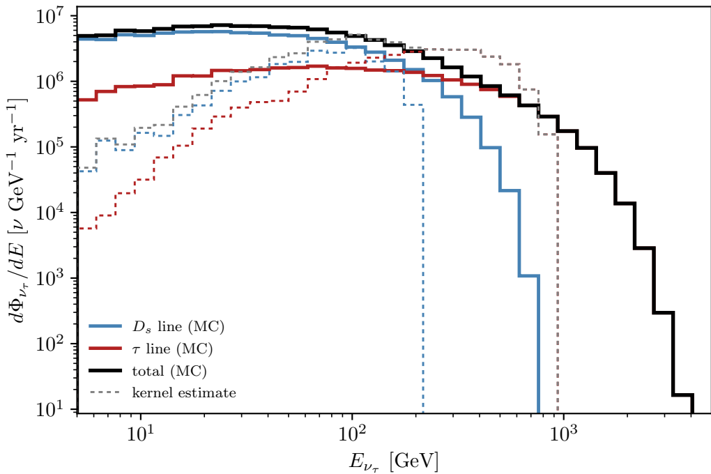
Secondary \nu_\tau flux: dimuon-inspired MC vs kernel
