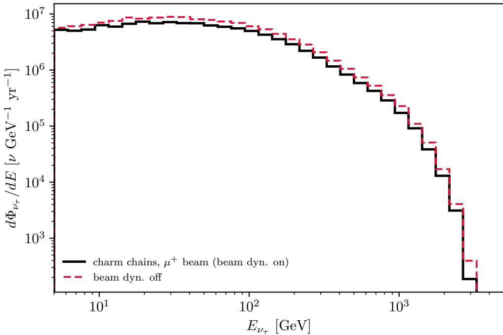
Secondary \nu_\tau flux at 5 km: beam dynamics on vs off
