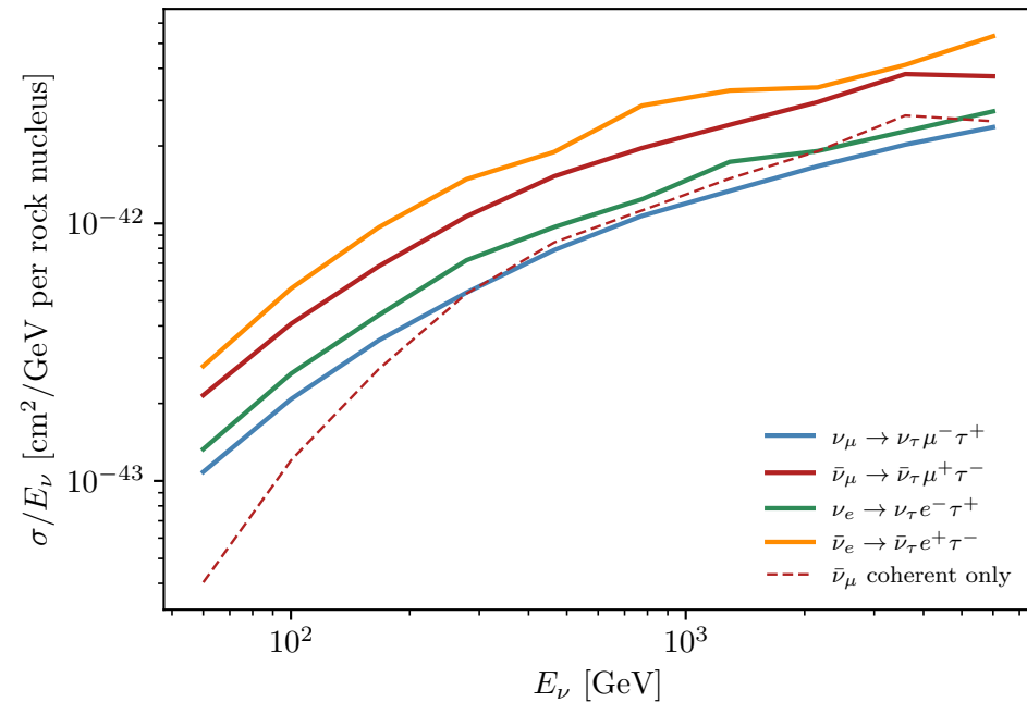
\ell\tau trident cross sections, rock ( Z = 11, A = 22 )
