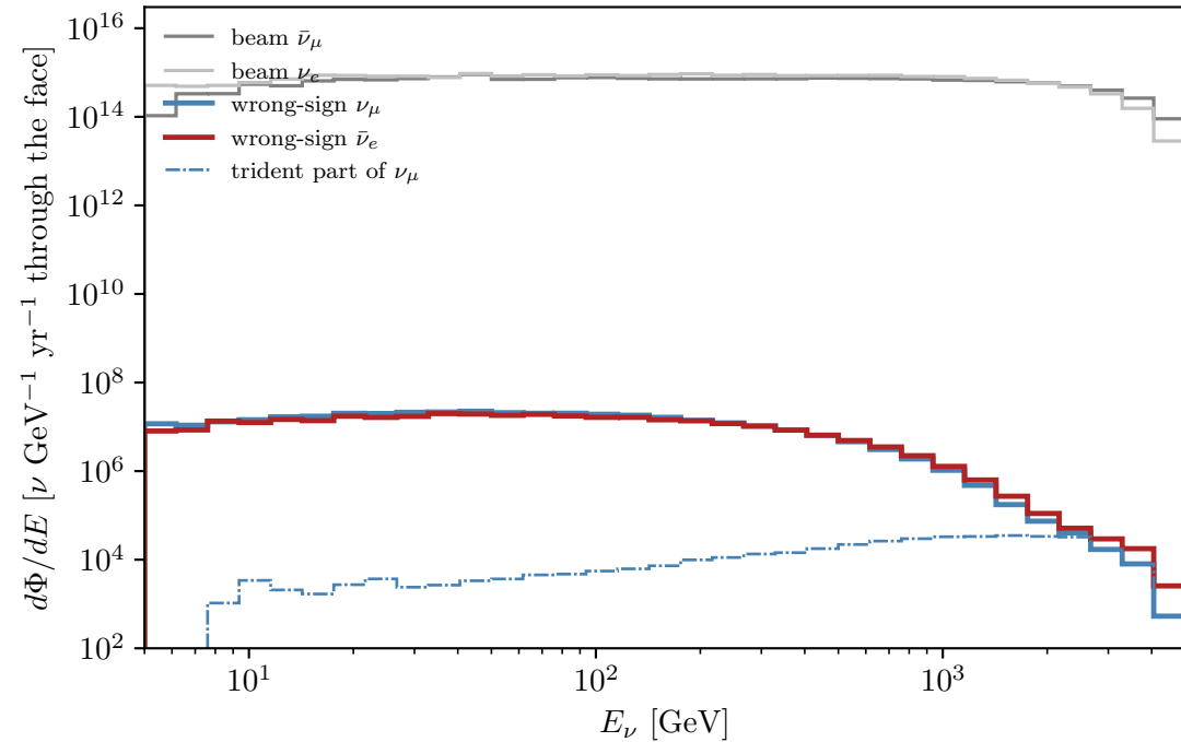
\mu^+ beam (downstream det.)
