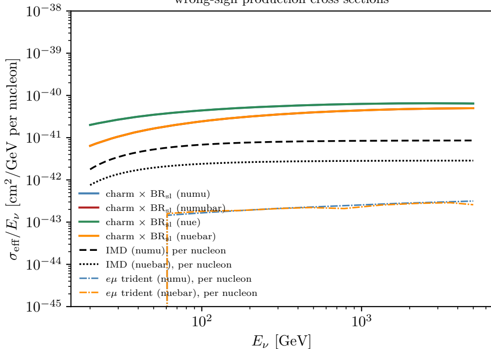
wrong-sign production cross sections
