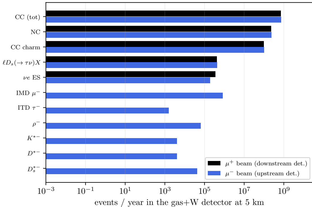
SM event rates by channel
