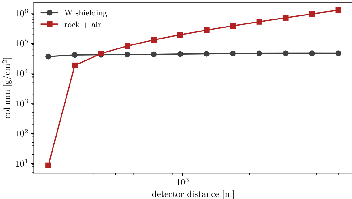
Flux-weighted material in front of the detector
