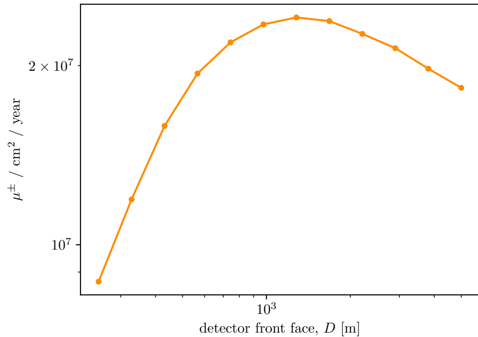
secondary muon flux density
