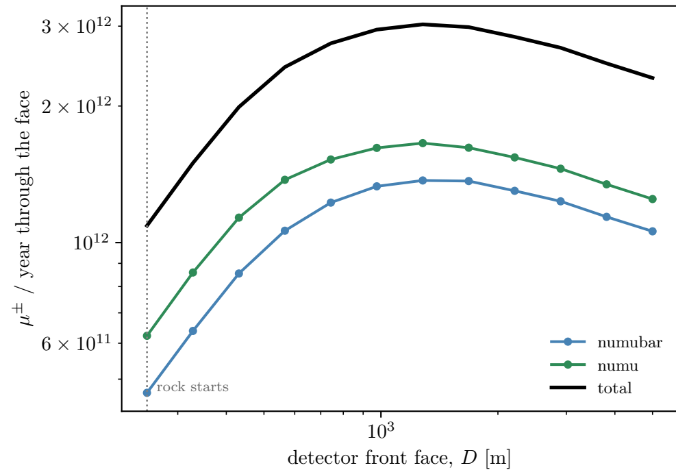
Milestone 2: secondary muons vs detector location
