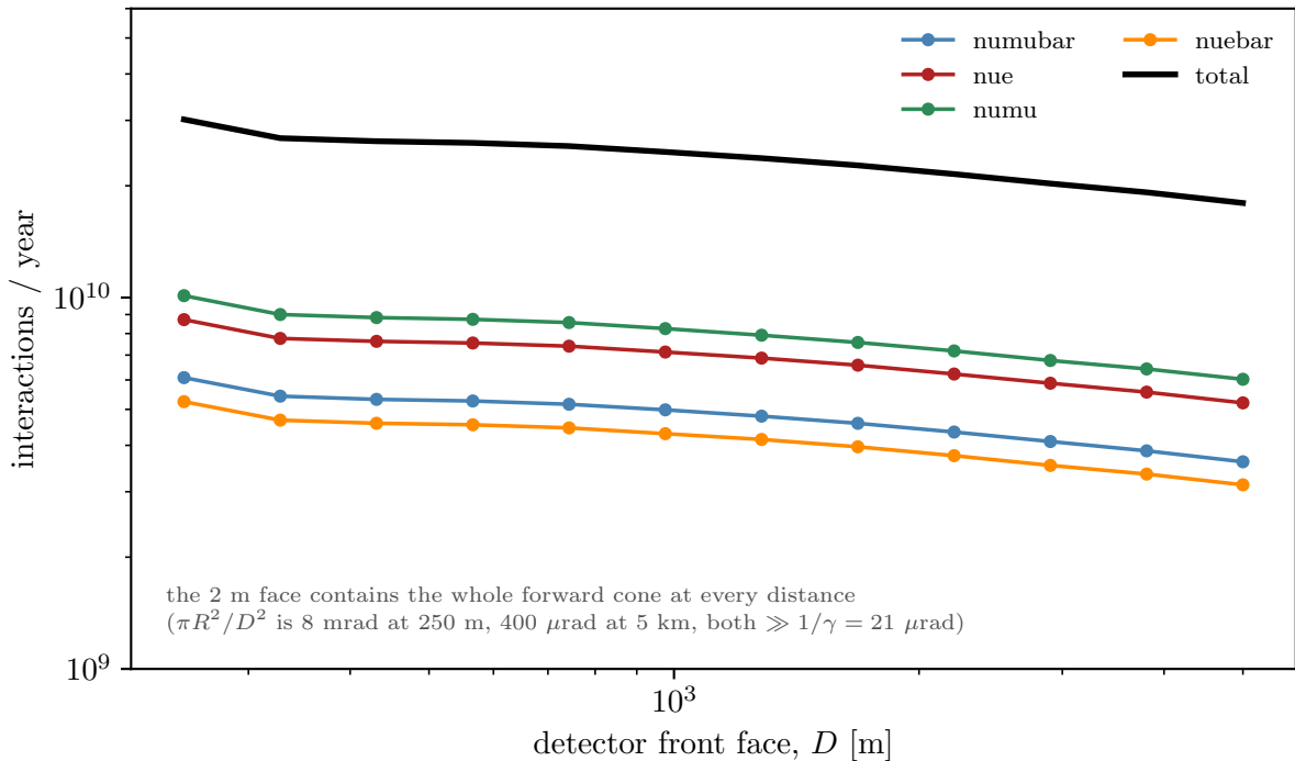
Milestone 1: SM neutrino interactions vs detector location (both beams, HPGAr + 3 W slabs, r = 2 m)
