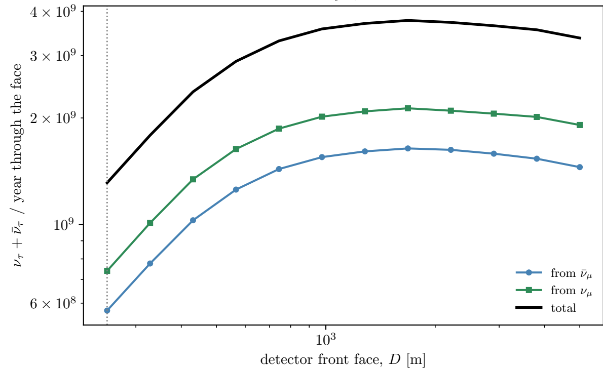
Milestone 3: secondary \nu_\tau vs detector location
