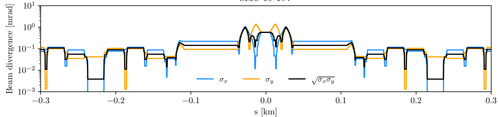
MuC-10-TeV
