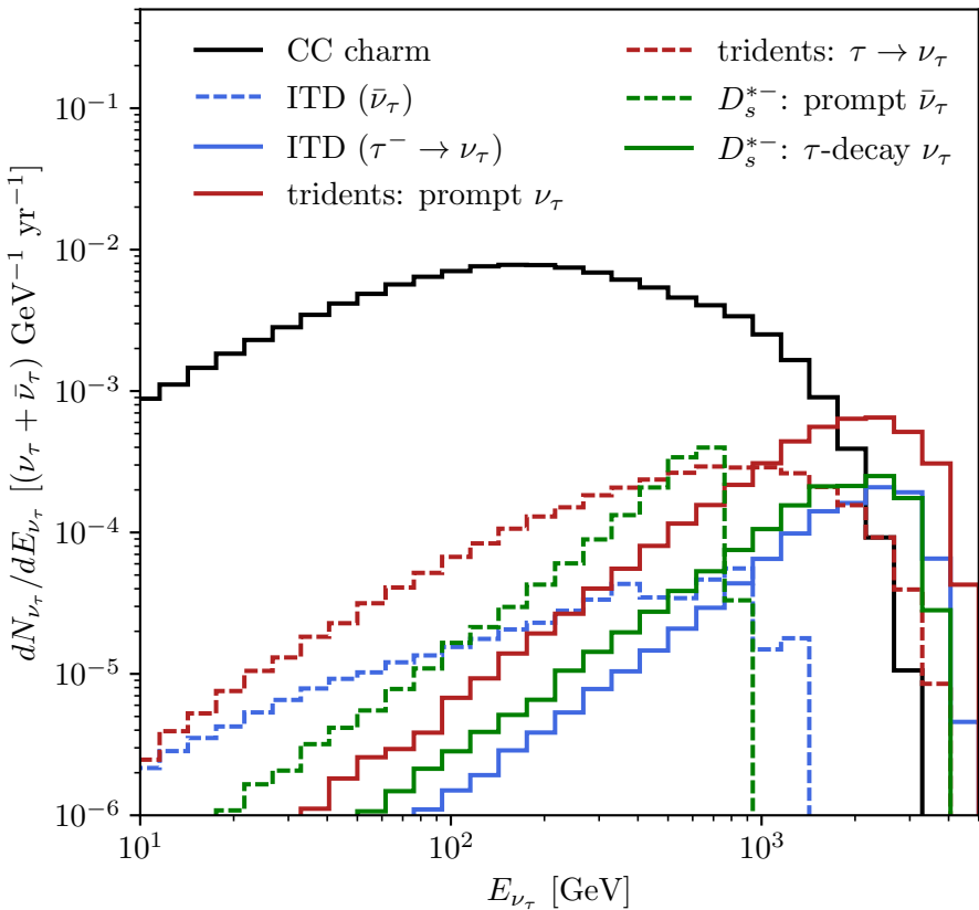
\ell\tau -trident \nu_\tau vs the other sources
