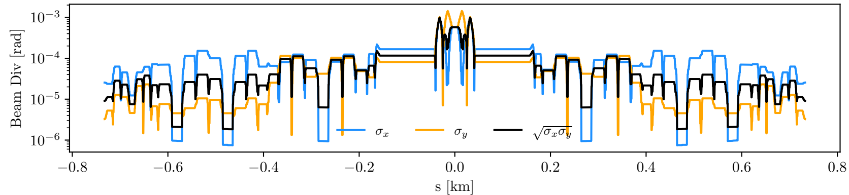
MuC-10-TeV-curves
