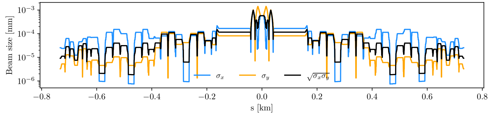
MuC-10-TeV-curves
