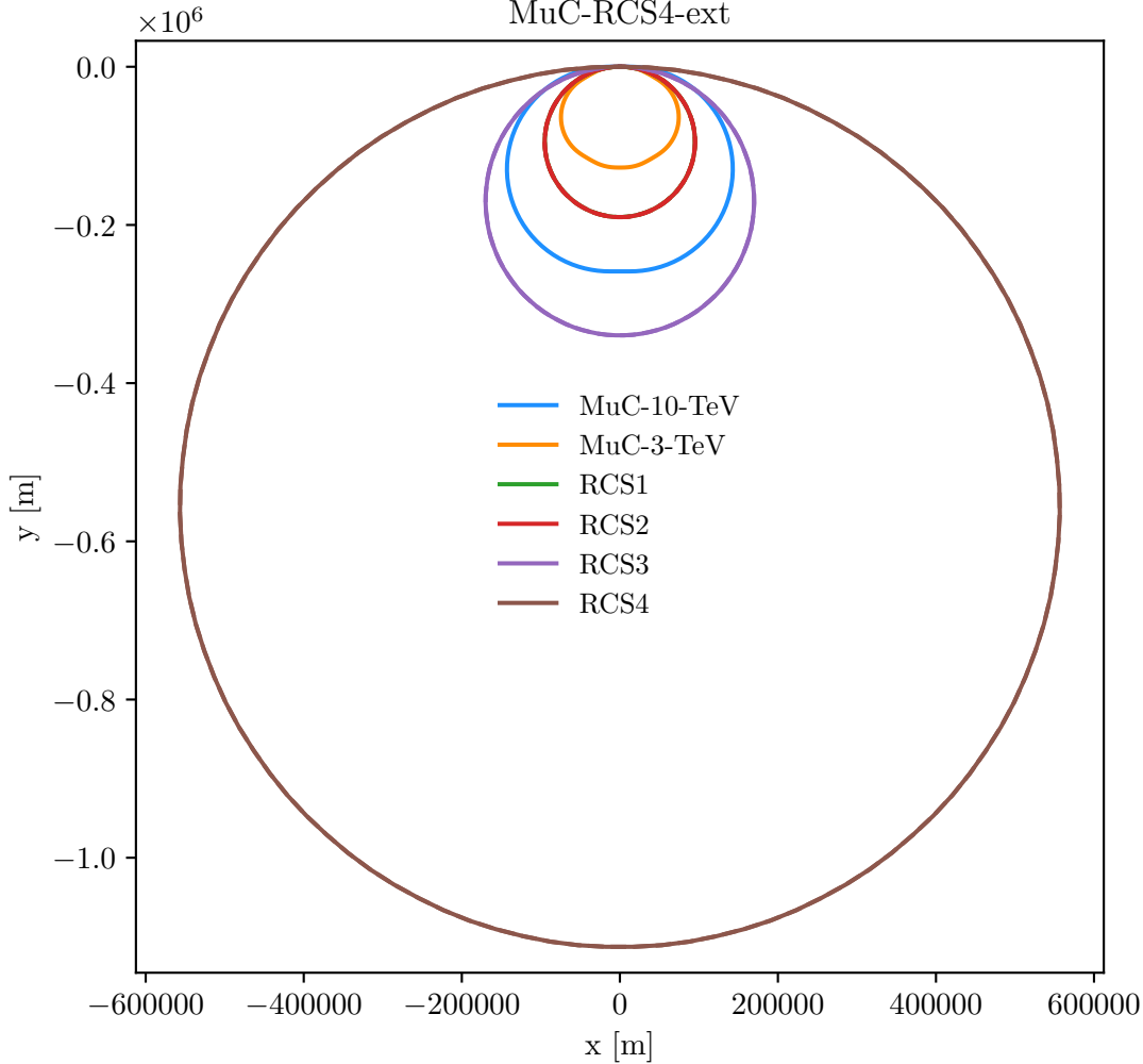
MuC-RCS4-ext
