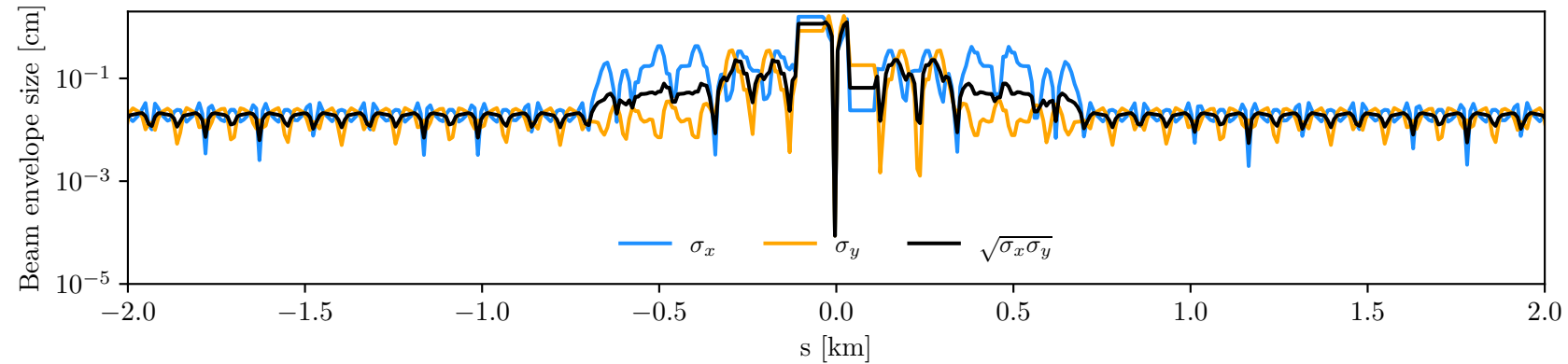
MuC-10TeV
