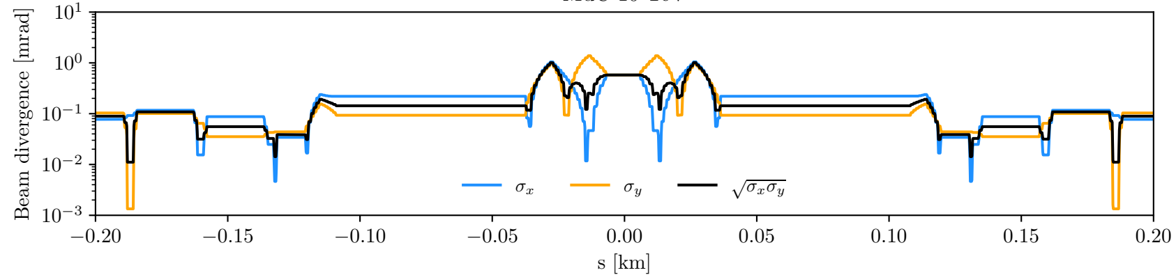
MuC-10-TeV
