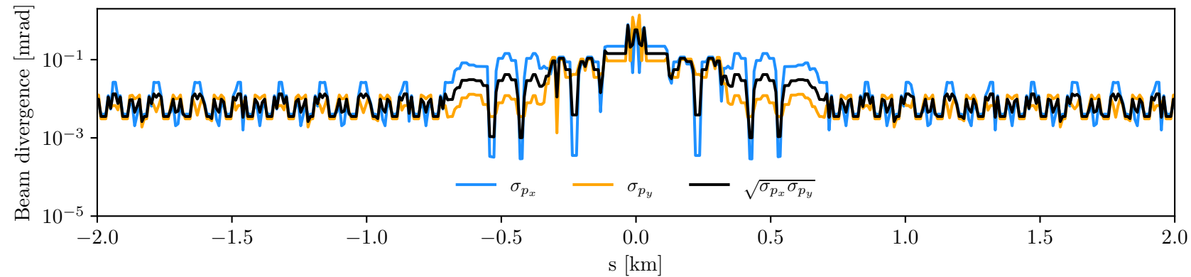
MuC-10TeV
