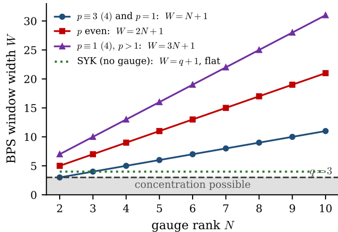
(a) gauge models vs. SYK
