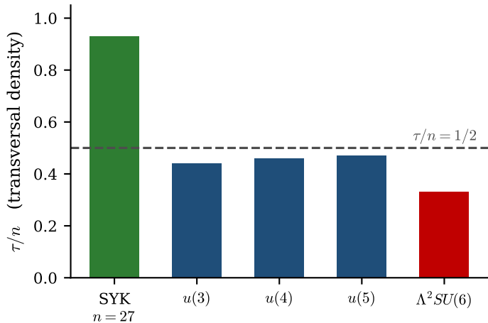
(b) \tau/n \rightarrow 1 concentrates, \leq 1/2 obstructed
