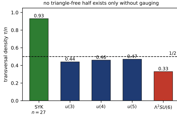
Figure 5: Transversal densities. SYK approaches 1, since no triangle-free set exceeds q - 1 ; gauge models sit near \frac{1}{2} , the positive-root half; two-index antisymmetric matter is worse still. This density governs (28); the window itself is set by the symmetry class (§5).
