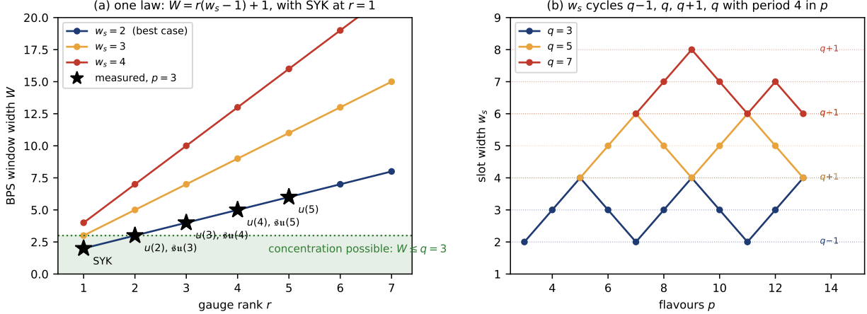
Figure 2: (a) The rank law with the measured models on it; SYK is not a separate case but the point r = 1 . (b) The slot width for generic couplings, cycling through q - 1, q, q + 1, q with period four in p as the bilinear form (15) alternates between symmetric and antisymmetric.
