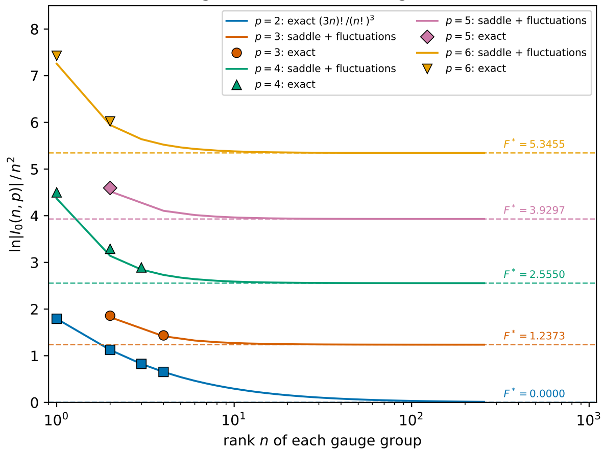
(c) leading large- n coefficients
