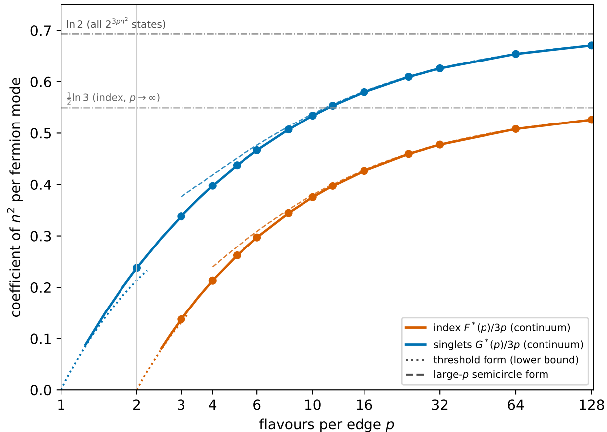
(c) leading large- n coefficients
