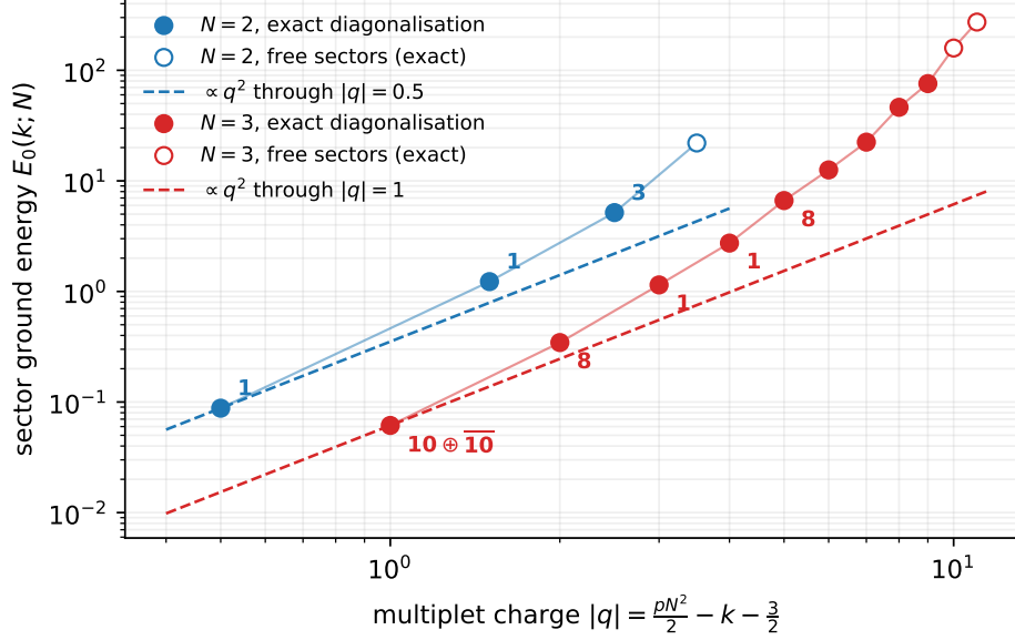
Figure 8: Sector ground energies below the window against the multiplet charge |q| of (17), at N = 2 and 3 , from exact diagonalisation of the zero-weight block of each sector. Open circles are free sectors, given exactly by (15). The dashed lines are the super-Schwarzian law E_0 \propto q^2 , drawn through the point nearest the window. The labels give the irrep of each ground state near the window.
