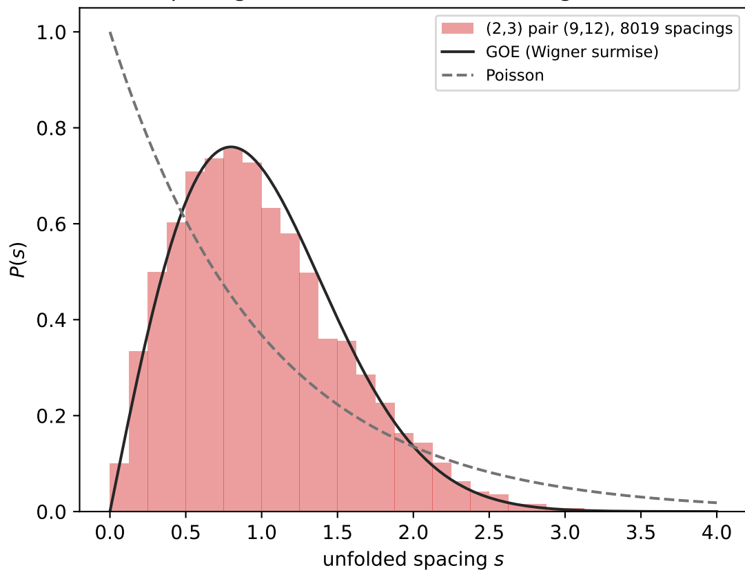
(c) spacing distribution (local unfolding, \pm 8 levels)
