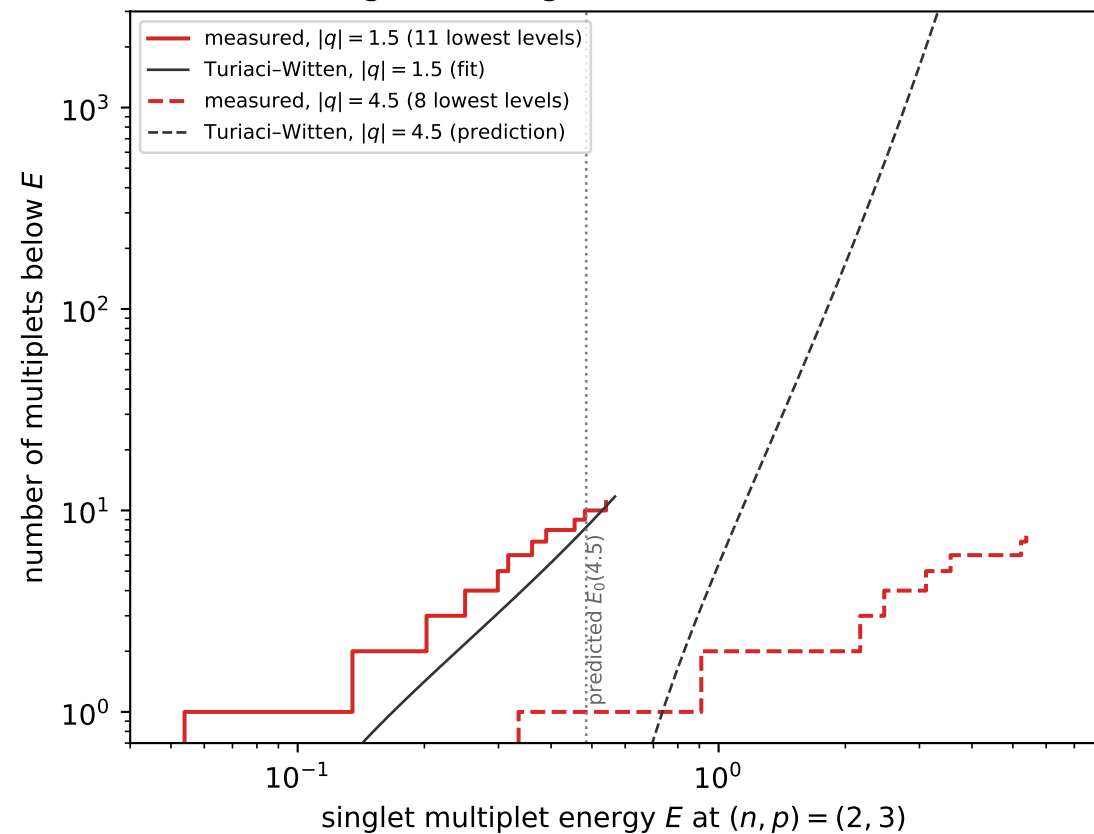
(d) near-edge counting vs Turiaci-Witten ( E_s=0.862 )
