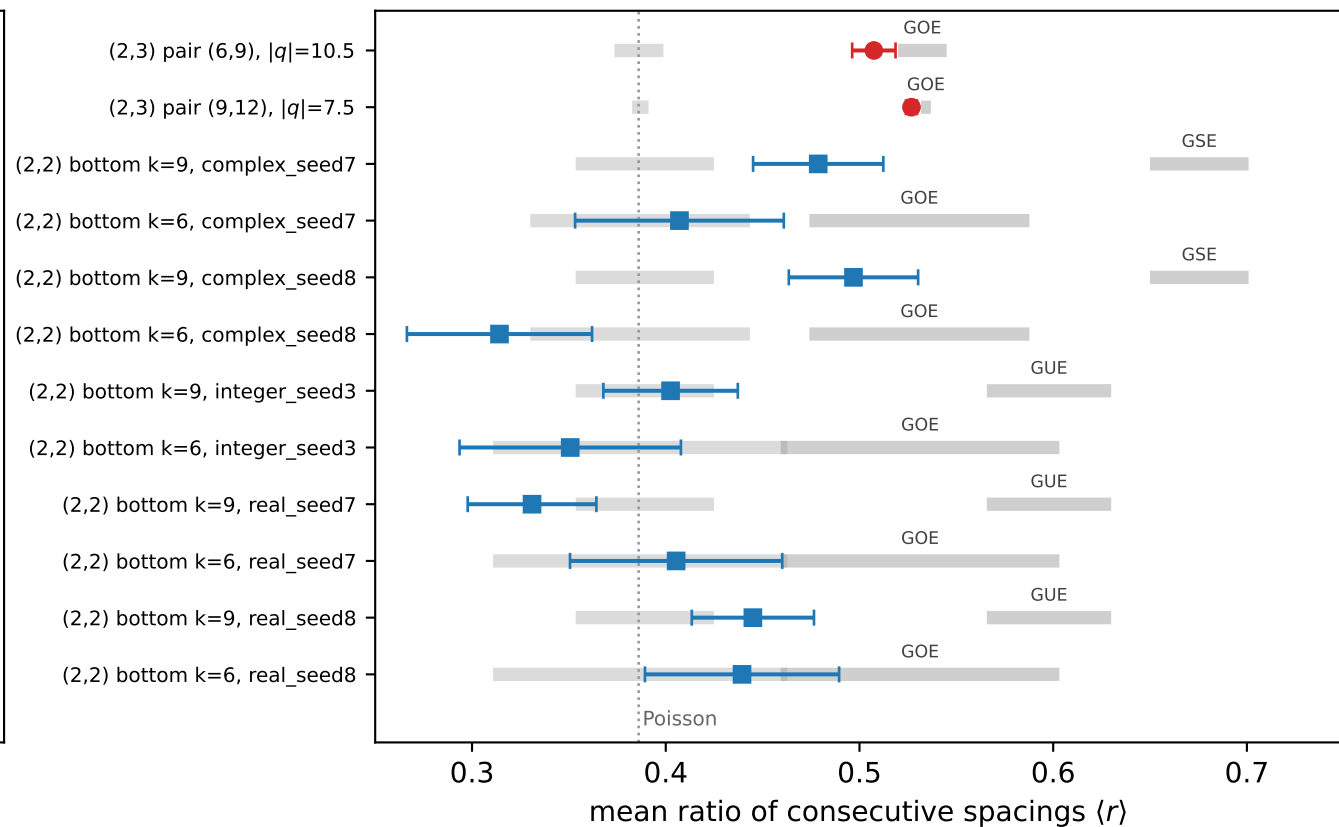
(b) level statistics (bars: size-matched references)
