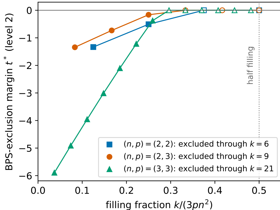
(a) singlet BPS exclusion: t^* < 0 means no BPS singlet at degree k
