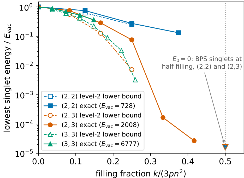
(b) singlet gap per degree: bootstrap bound vs exact
