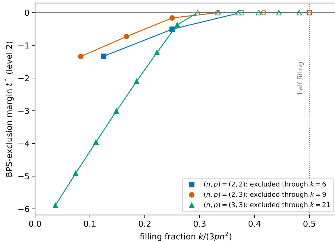
(a) singlet BPS exclusion: t^* < 0 means no BPS singlet at degree k
