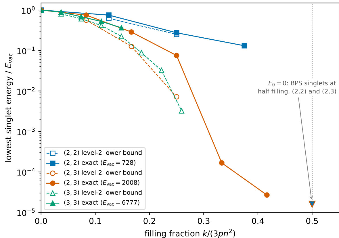
(b) singlet gap per degree: bootstrap bound vs exact
