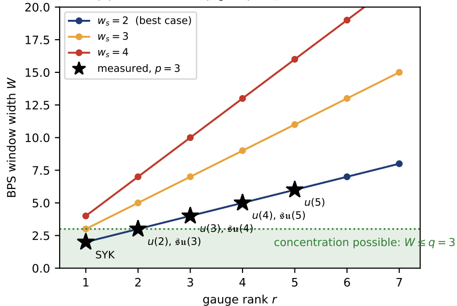
(a) one law: W = r(w_s - 1) + 1 , with SYK at r = 1
