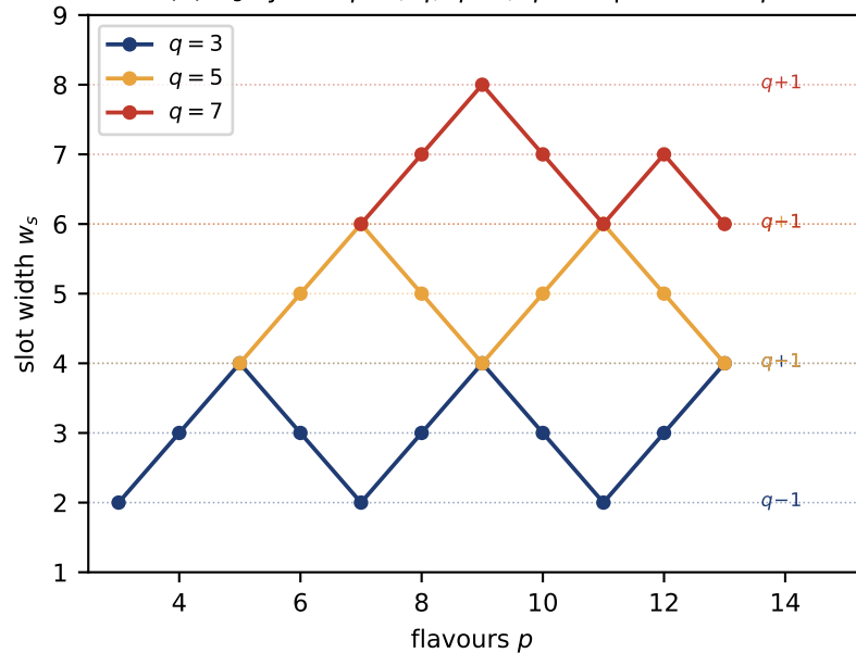
(b) w_s cycles q-1, q, q+1, q with period 4 in p
