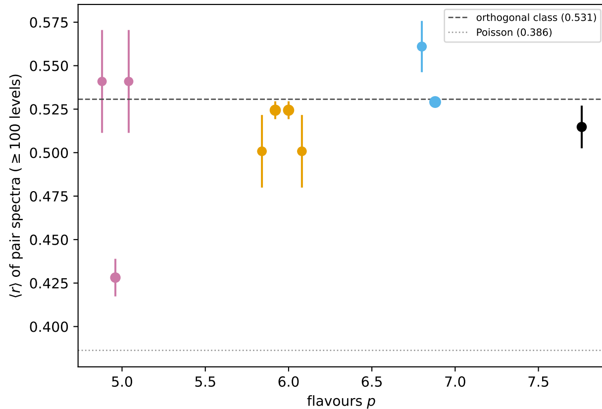
(c) n = 1 : level statistics per multiplet sector
