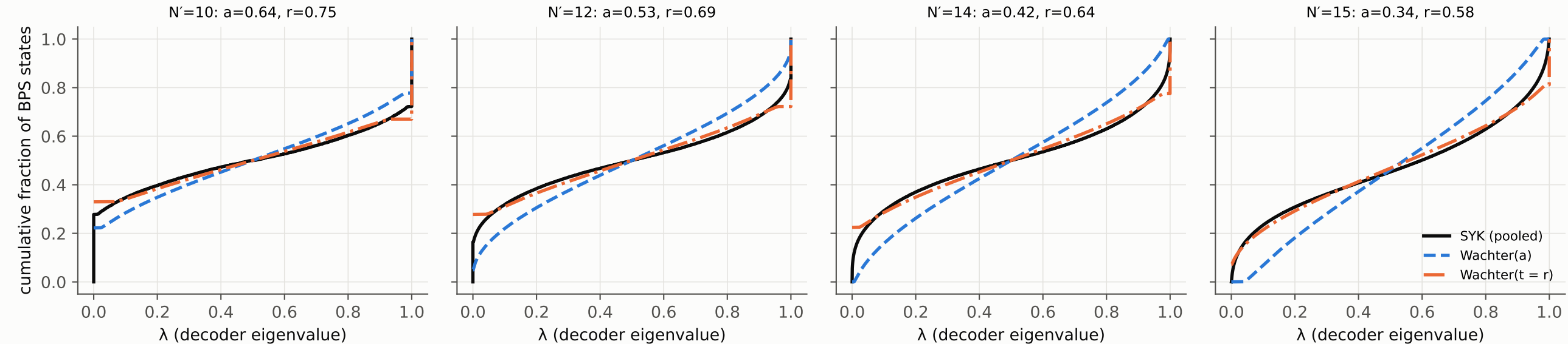
Decoder spectra ( q=3 ): Wachter( t=r ) matches the moments but puts wall mass in atoms; SYK spreads it continuously
