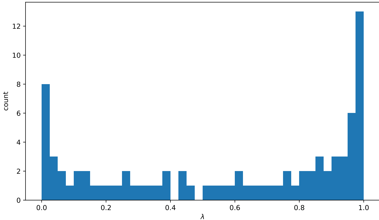
K_T spectrum: N = 9 \rightarrow 10 , p = 4 , down channel
