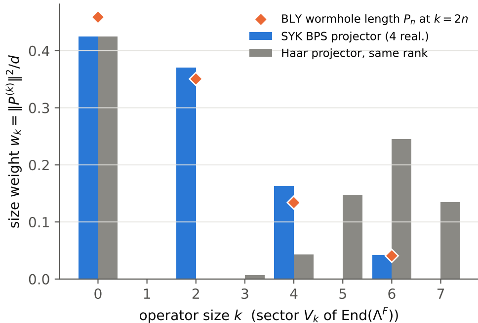
(a) size spectrum of P , N' = 14 ( w_0 = a exactly)
