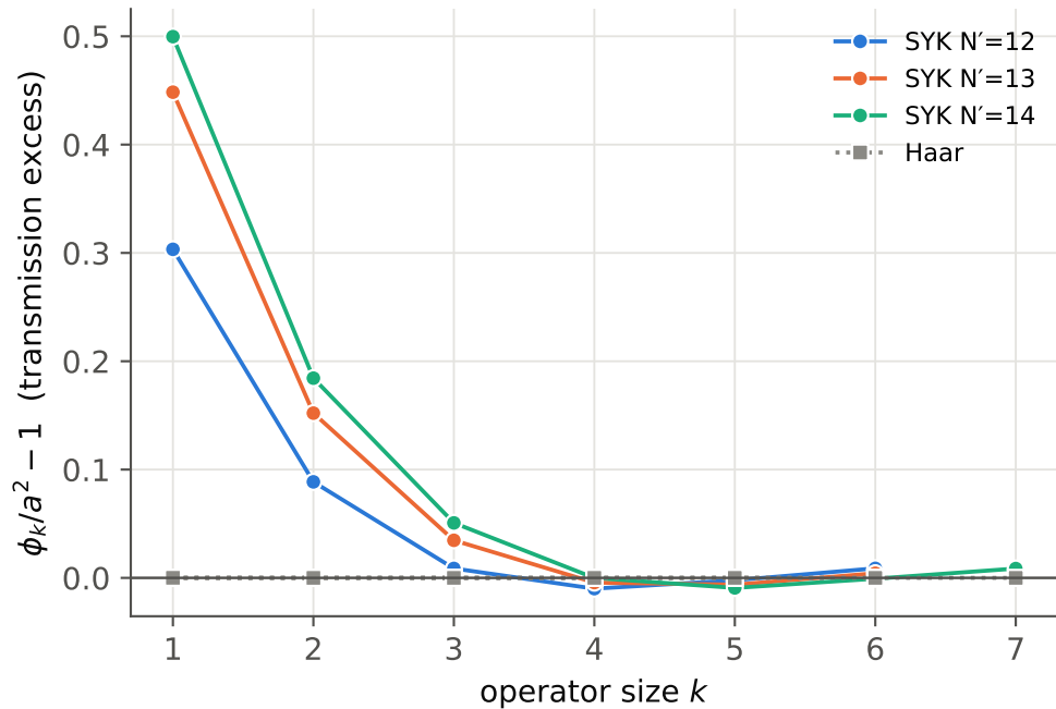
(b) transmission X \mapsto E[XPX] on V_k : free \leftrightarrow flat
