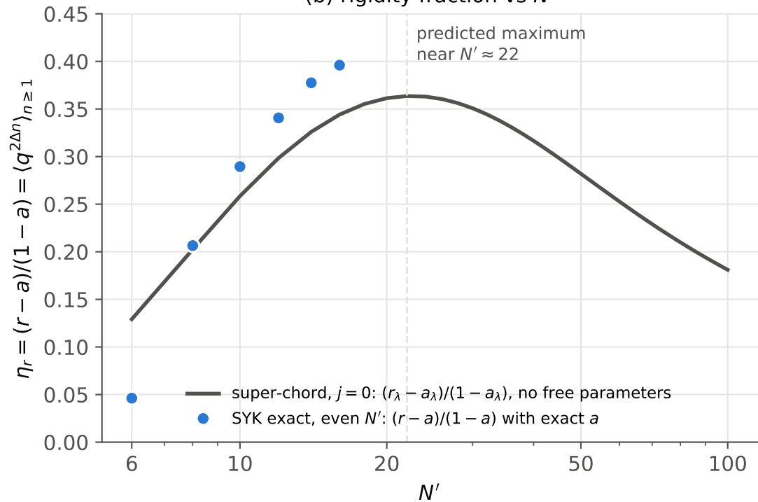
(b) rigidity fraction vs N'
