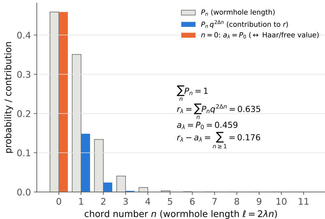
(a) SUSY wormhole at N' = 14 ( \lambda = 1.29 , j = 0 , \Delta = 1/3 )
