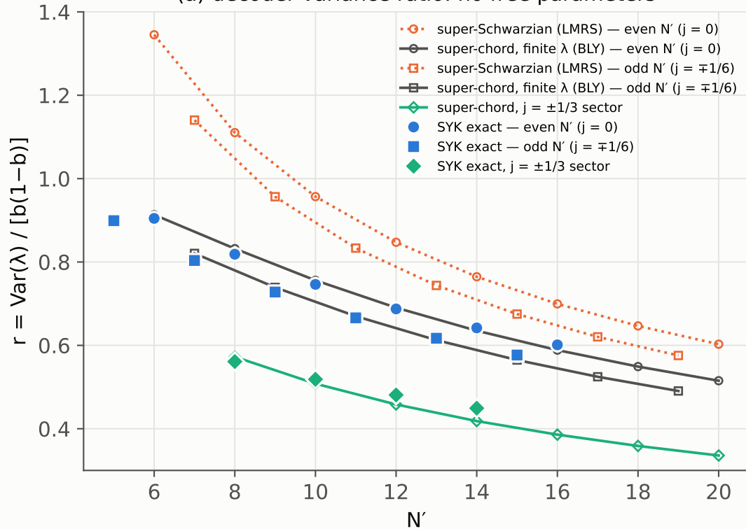
(a) decoder variance ratio: no free parameters
