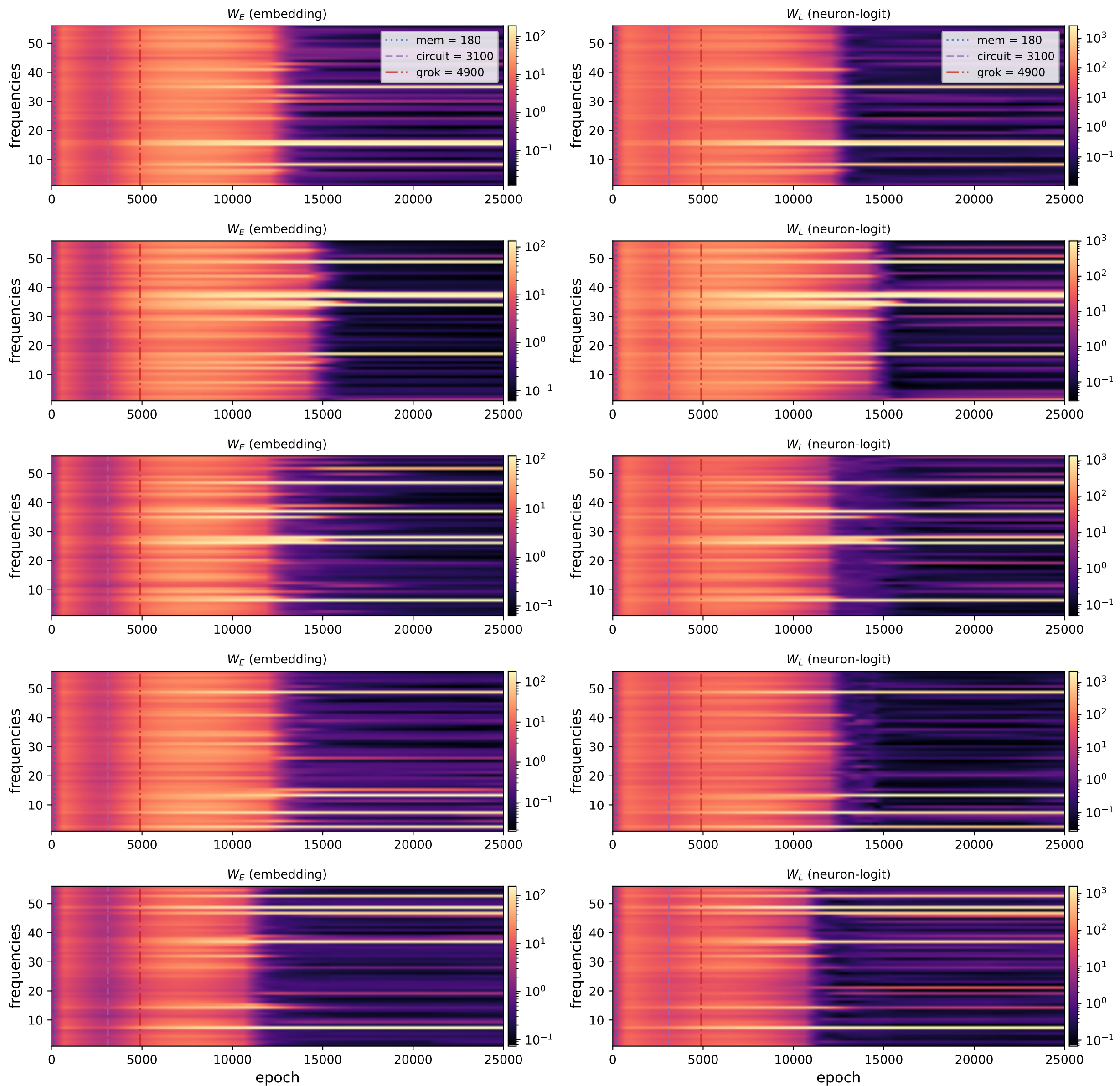
Phase 2 - EGD m=0 slow (lr=0.01, wd=0.1) - frequency masses (per seed) · n=5 seeds (one row each)
