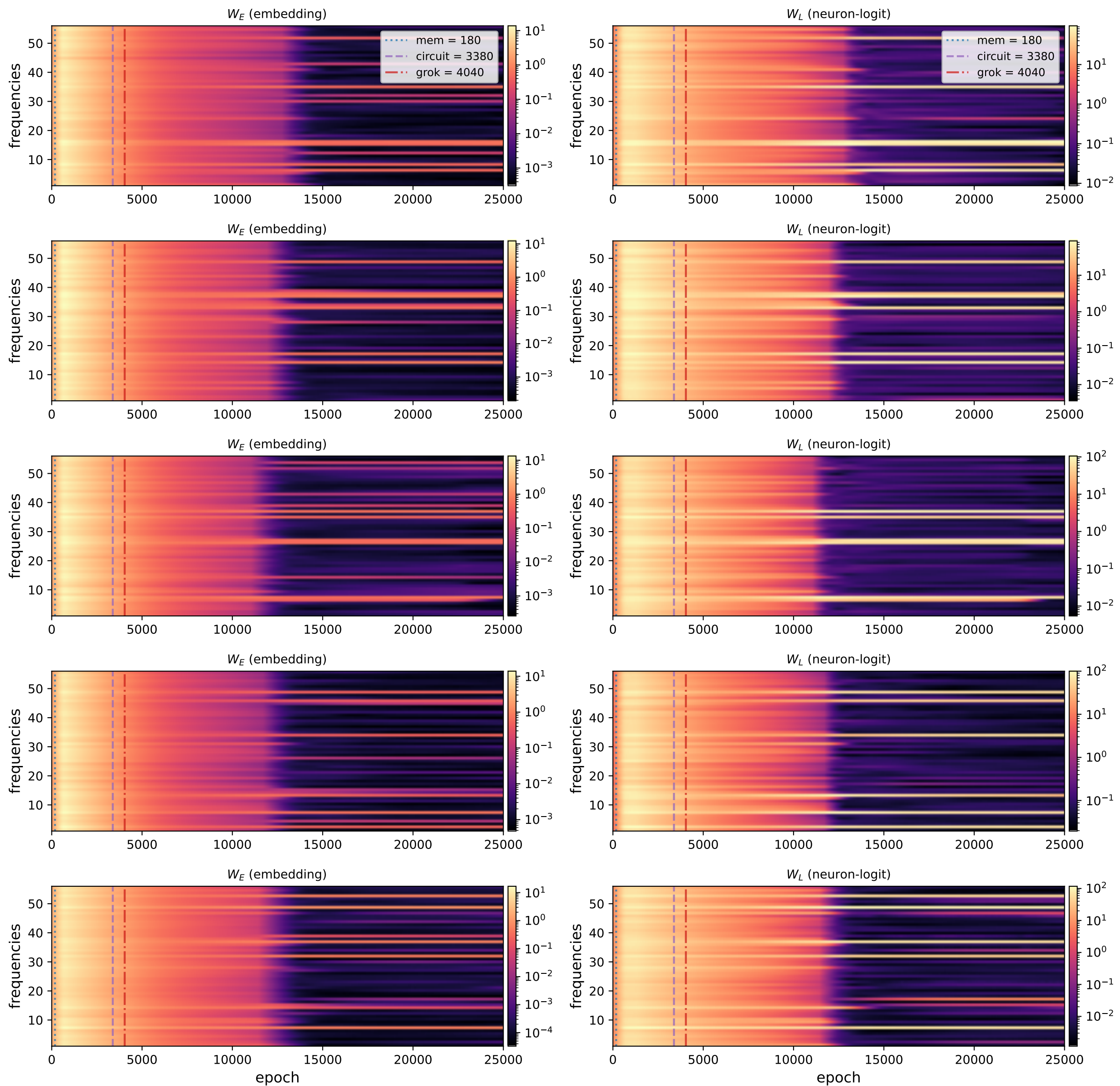
Phase 2 - Muon m=0 slow (lr=0.01, wd=0.1) - frequency masses (per seed) · n=5 seeds (one row each)
