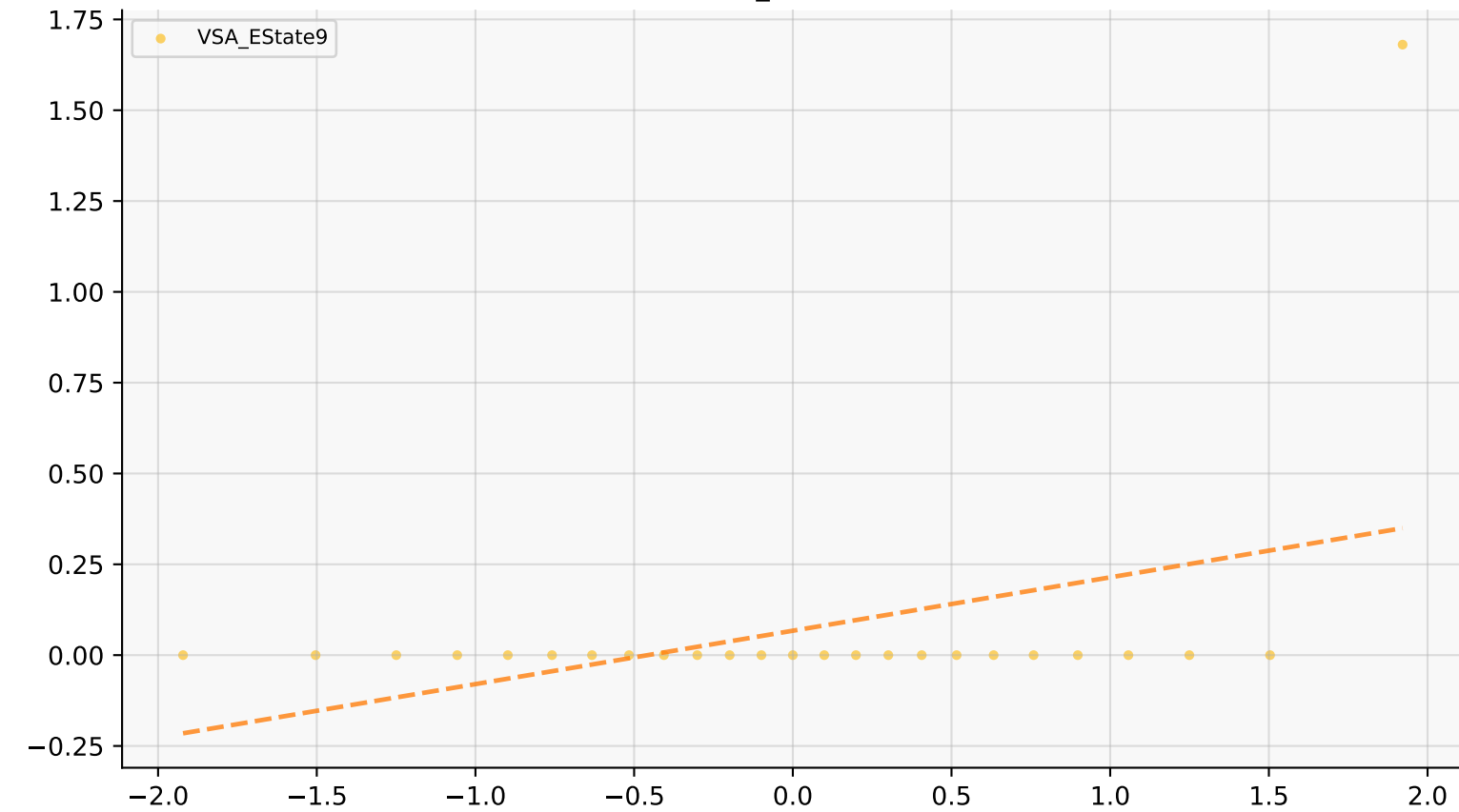
Morgan_r2_817
