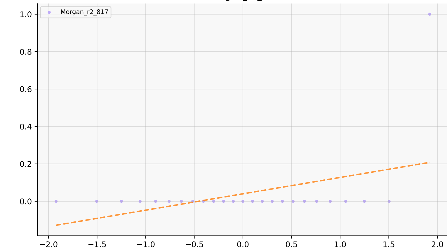
Morgan_r2_817
