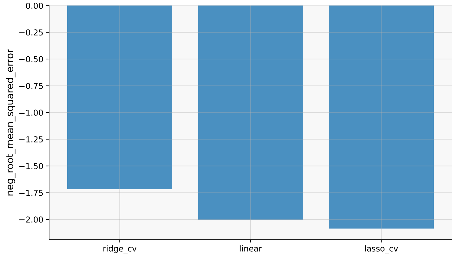
neg_root_mean_squared_error
