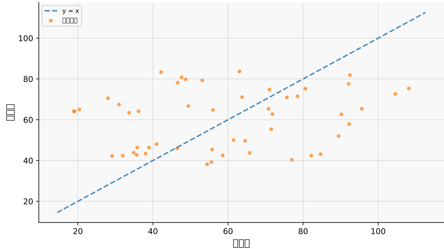
ridge vs (ridge_cv) n=50
