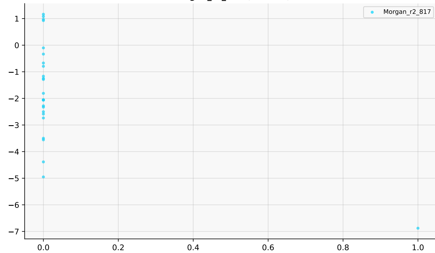
Morgan_r2_817 (r=-0.54)
