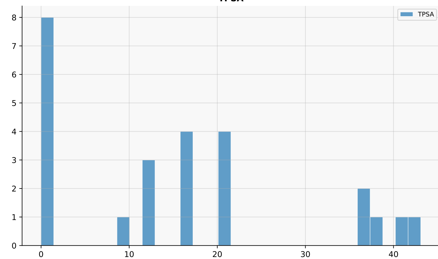
TPSA
