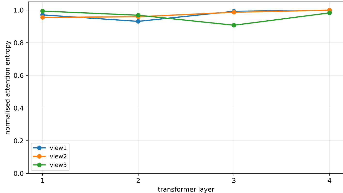
CIC-DDoS2019 - attention concentration by depth, seed 123 1.0 is uniform across features; lower means the view has specialised
