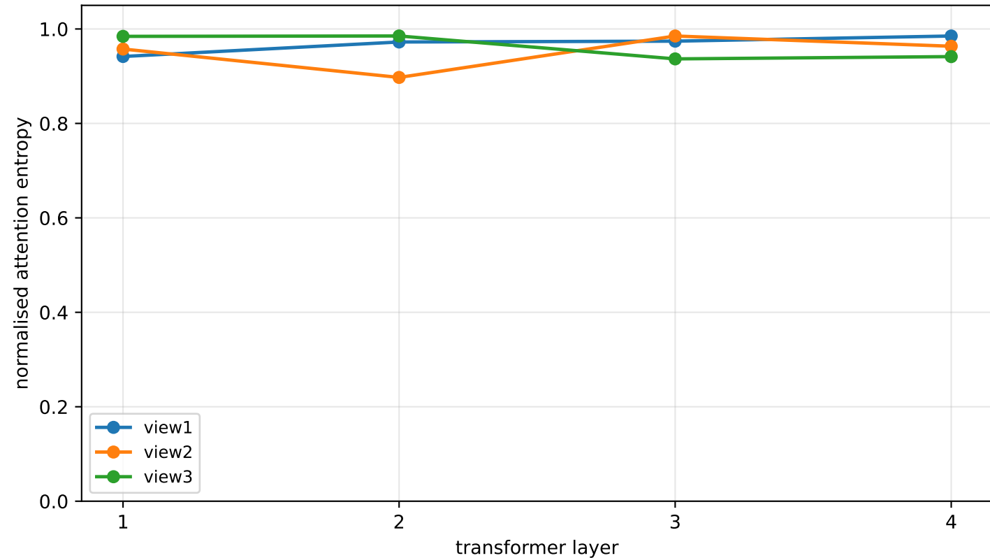
CIC-DDoS2019 - attention concentration by depth, seed 42 1.0 is uniform across features; lower means the view has specialised
