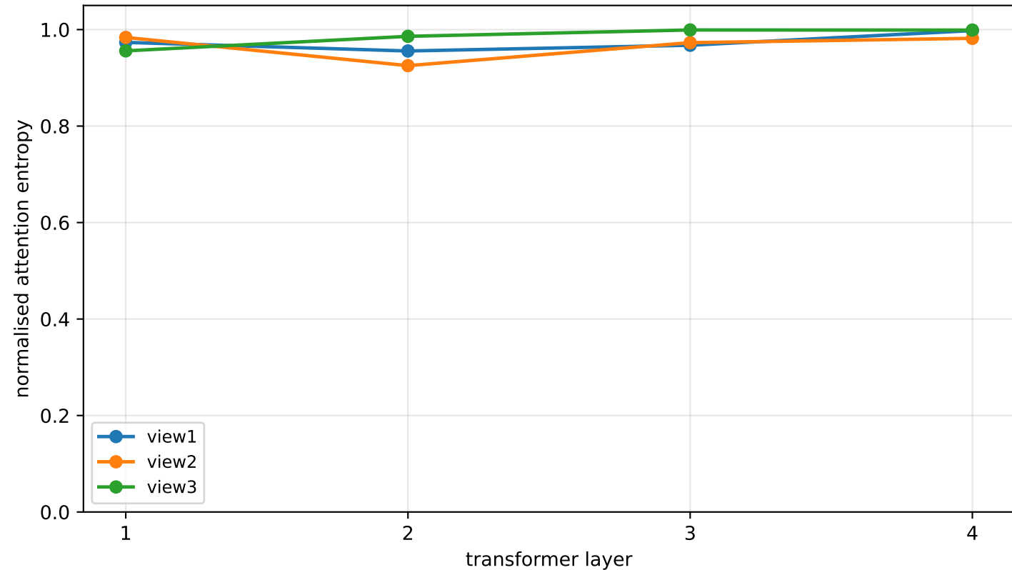
CIC-DDoS2019 - attention concentration by depth, seed 456 1.0 is uniform across features; lower means the view has specialised
