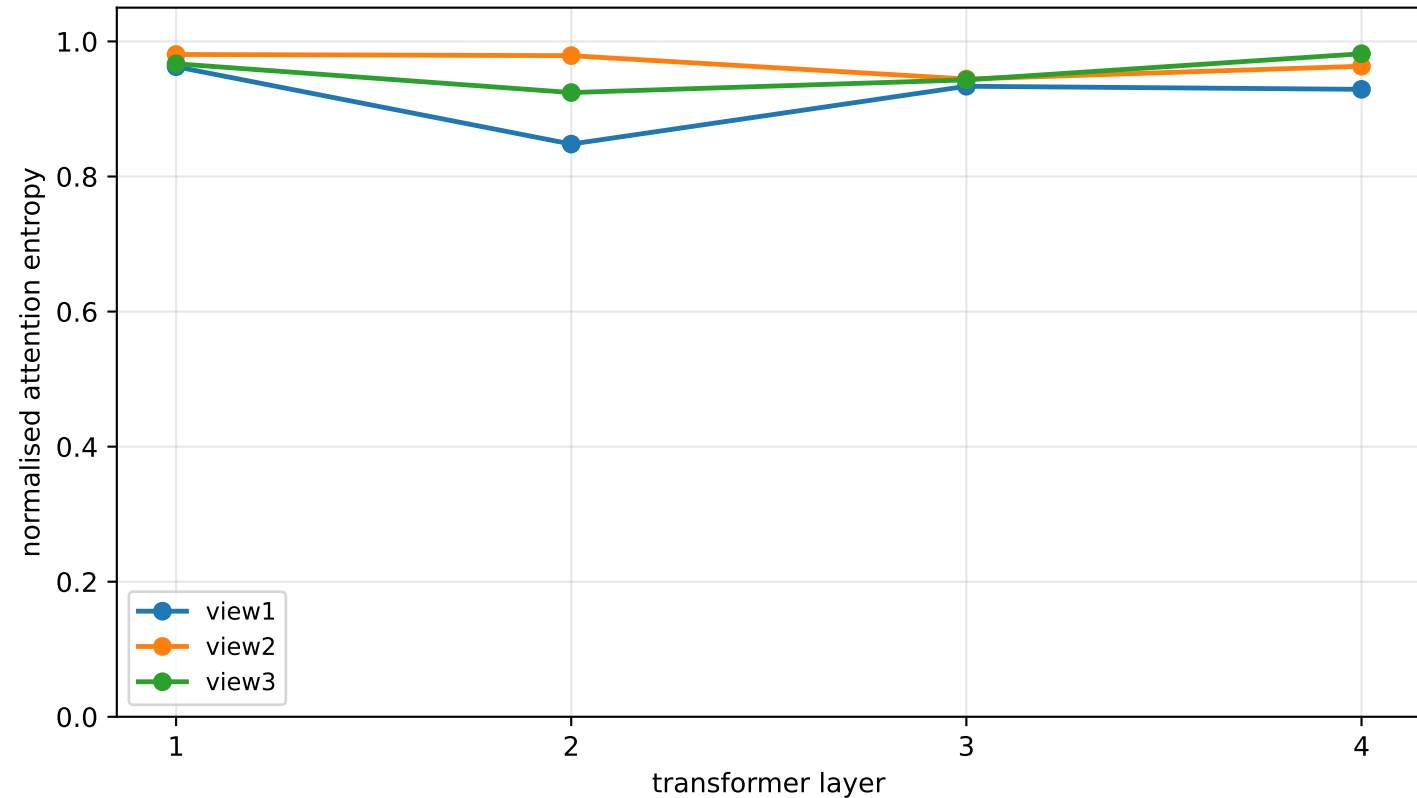
CIC-IDS-2017 - attention concentration by depth, seed 123 1.0 is uniform across features; lower means the view has specialised
