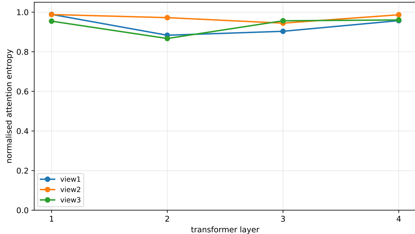
CIC-IDS-2017 - attention concentration by depth, seed 456 1.0 is uniform across features; lower means the view has specialised
