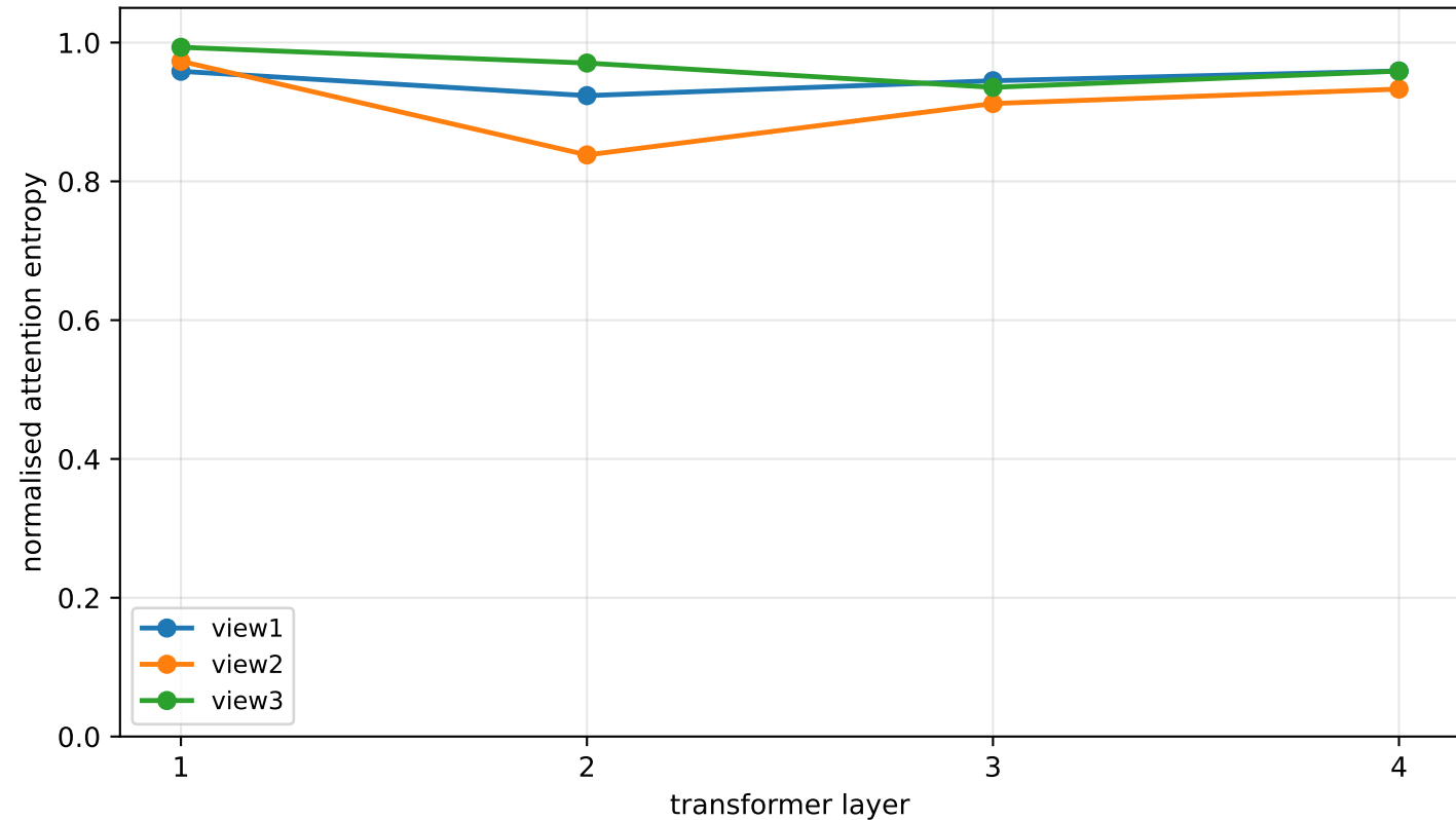
NSL-KDD - attention concentration by depth, seed 42 1.0 is uniform across features; lower means the view has specialised
